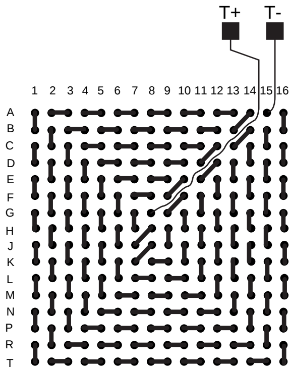
TEST VEHICLE BOARD
